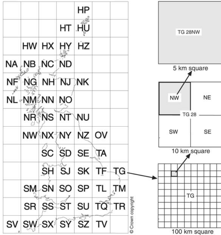
Figure 2 – Each NG square of 100 km by 100 km contains 400 (5 km by 5 km) squares. Land-Form PROFILE is supplied to customers in 5 km by 5 km tiles. These are referenced by NG letters followed by the appropriate numbers and figures which obey the 1:10 000 scale sheet numbering convention.
